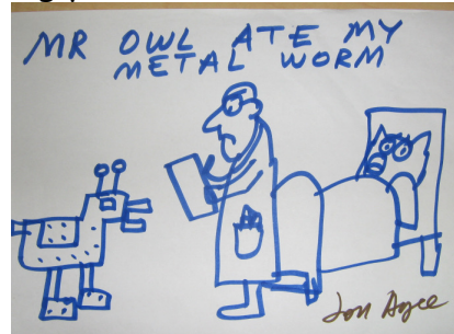
Another palindrome
